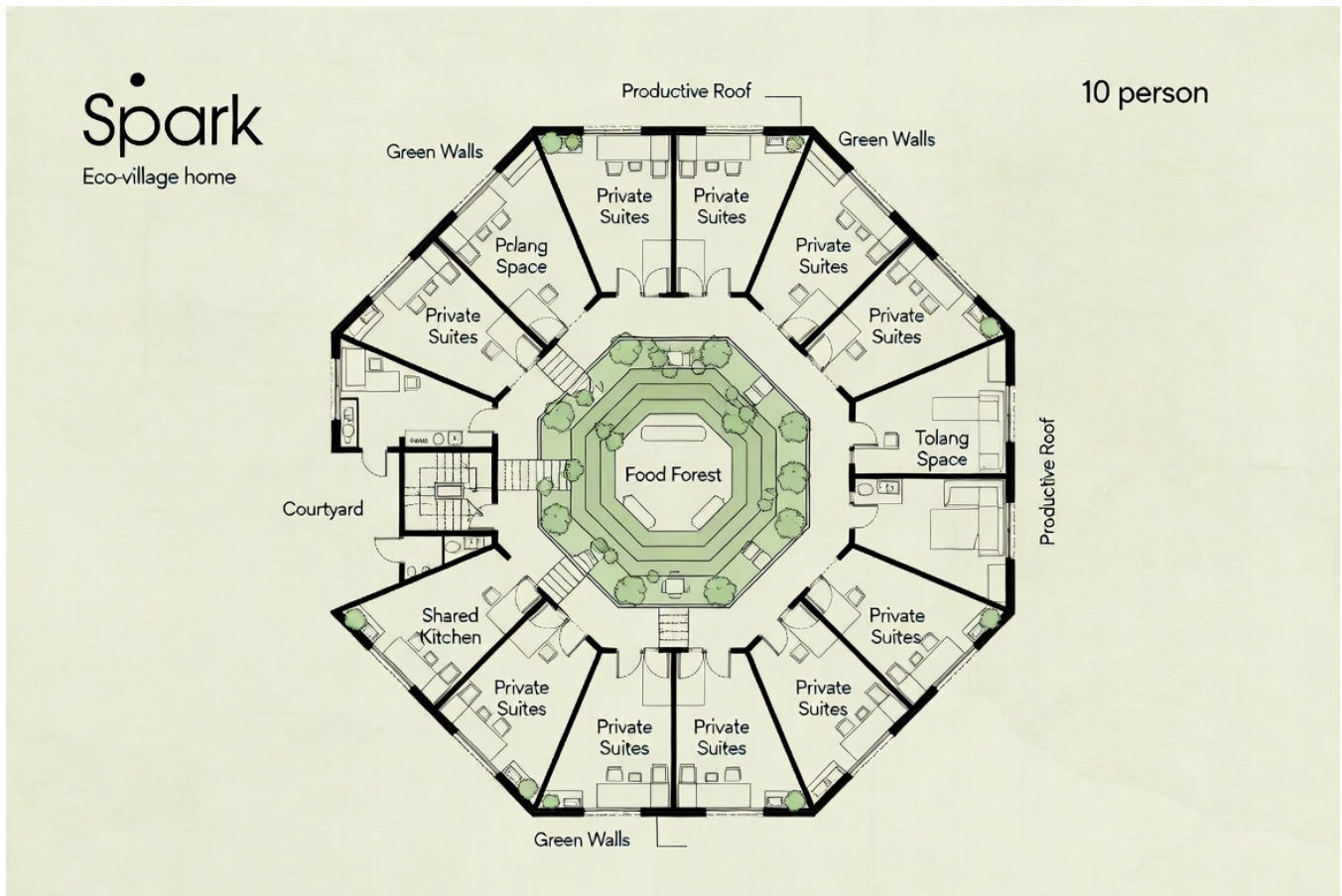
Figure 1: Spark Octagonal Courtyard Module Plan
